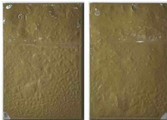
Figure 4 – Exfoliation failure of Cr-free Al-silicate basecoat, sealed with a Cr-free acid-phosphate topcoat in hot water immersion test.
