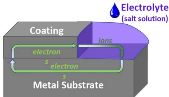
Figure 1 – Schematic of galvanically sacrificial coating.
