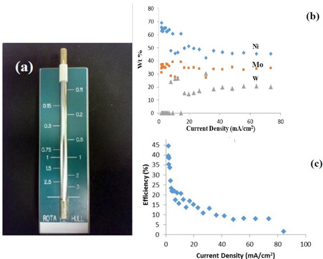
Figure 2 - Rotating Hull cell study of an electrolyte containing Ni, Mo and W at 500 rpm, at an average current density of 16.5 mA/cm 2 : (a) electrode and a scale representing a primary current distribution local current density estimate, (b) composition and (c) efficiency.
