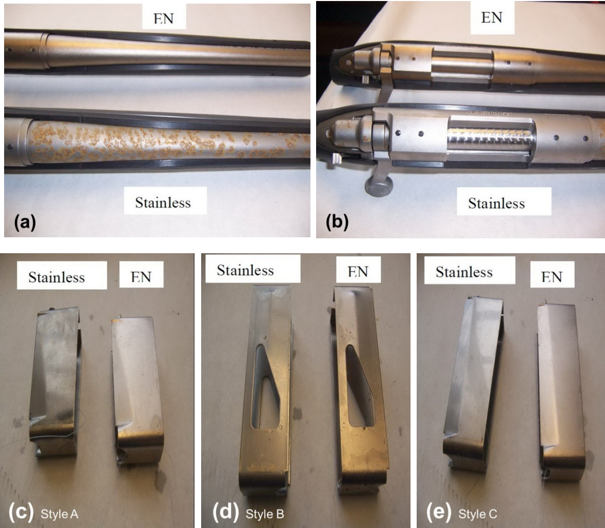
Figure 4 - Corrosion test results after 4 hours of salt spray: (a) barrels, (b) receivers, (c) magazine box style A, (d) magazine box style B and (e) magazine box style C. Both stainless and electroless nickel finishes are shown in each photo.
