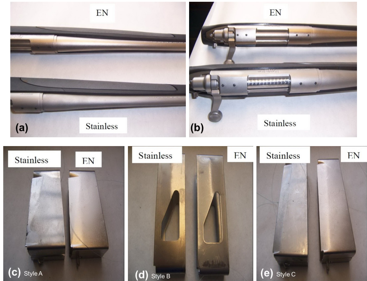
Figure 3 - Specimens under study in the as-received condition: (a) barrels, (b) receivers, (c) magazine box style A, (d) magazine box style B and (e) magazine box style C. Both stainless and electroless nickel finishes are shown in each photo.
